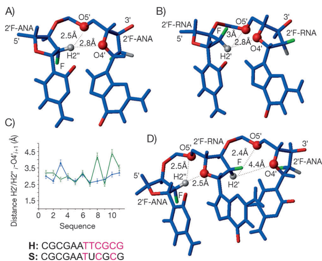
Figure 2. View of short distances between H2'/H2''...O4'/O5' oxygen atoms in A) 2'F-ANA and B) 2'F-RNA continuous tracts of H and S , respectively. C) Values of H2'/H2''...O4'_{i+1} distances all along the sequence (2'F-RNA in black and 2'F-ANA in magenta) in H (blue) and S (green). D) Structure and view of distances in steps of S . C blue, H gray, O red, F green.
